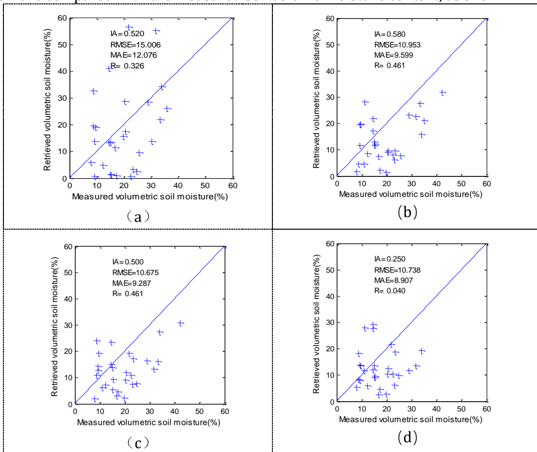
Figure 3 comparison between measured soil volumetric moisture content and inverted soil volumetric moisture content under different filter window sizes: a (1*1), b (3*3), c (5*5), d (7*7)
